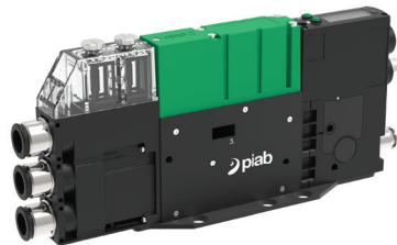
piCOMPACT®23 SMART Single unit with large filter
