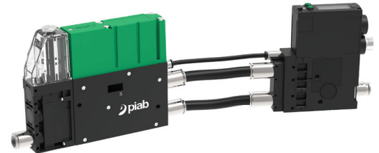
piCOMPACT®23 SMART Split units
